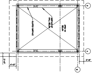
3 UPPER CLOSETORY PLAN
